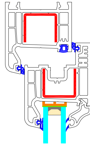
A-1 Detail
